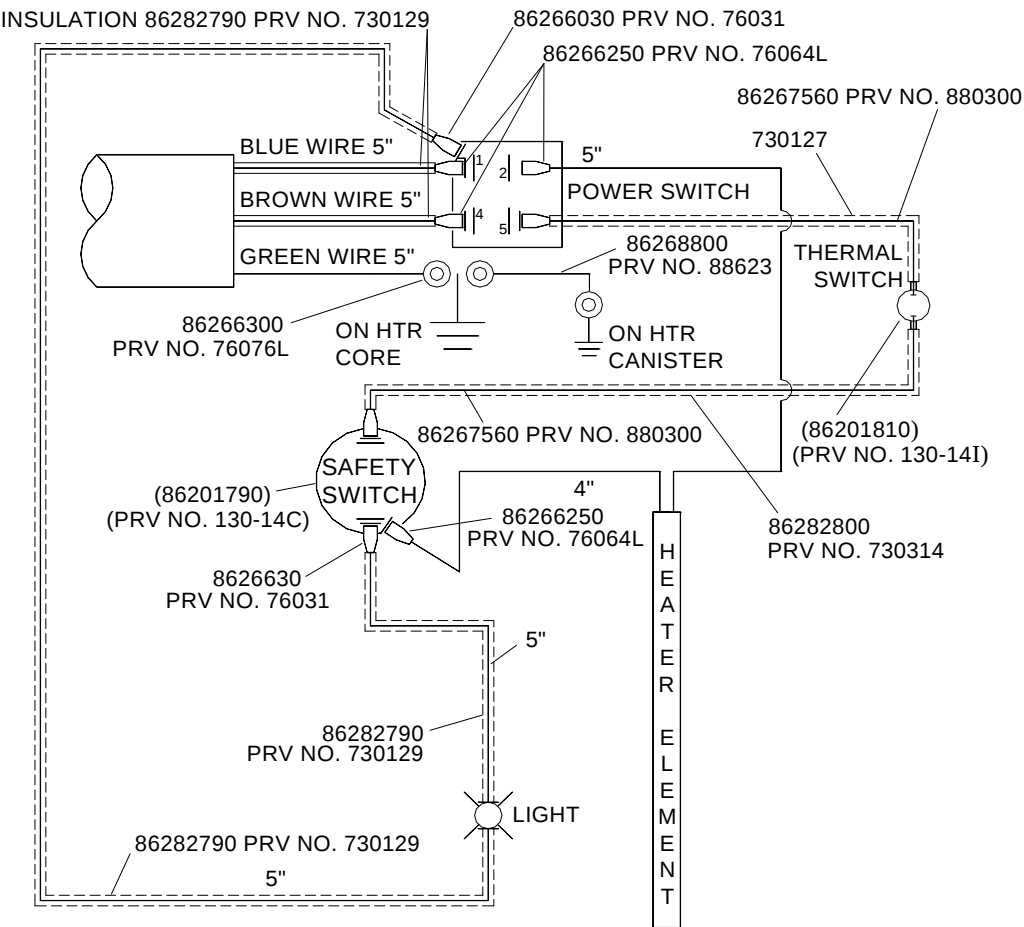
PRO HEATER DIAGRAM
