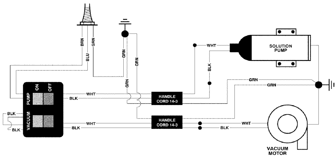
WIRING DIAGRAM, 240V EMC MODEL
