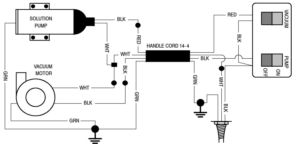
WIRING DIAGRAM, 220V/230V
