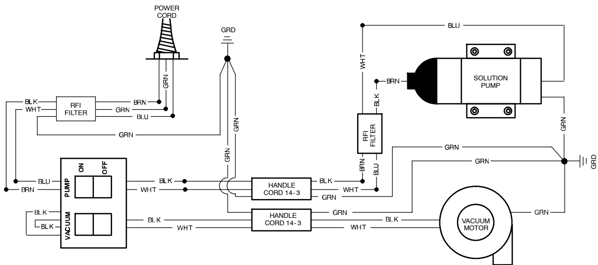
WIRING DIAGRAM, 240V EMC MODEL
