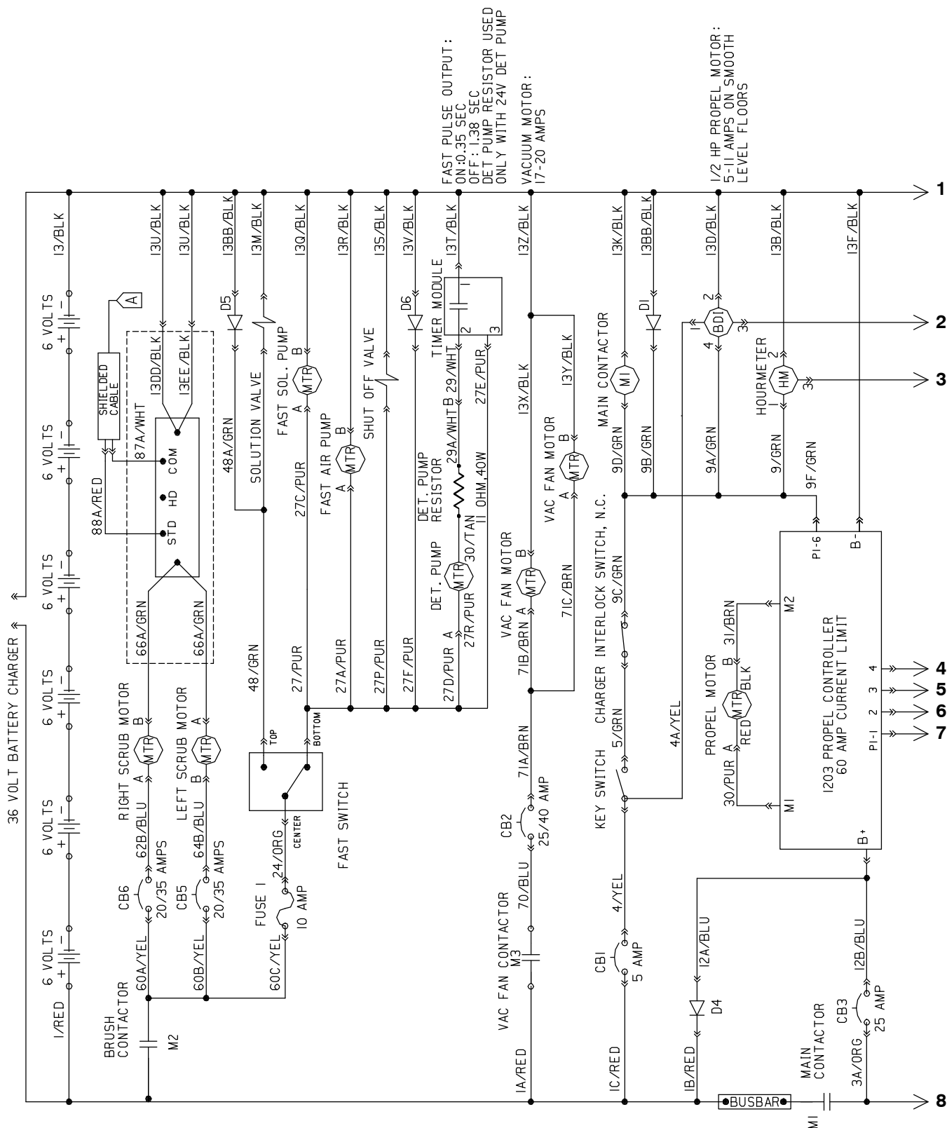
Fig. 38 – Electrical Schematic, Standard & Fast Model (S/N 10000000–10741220)
