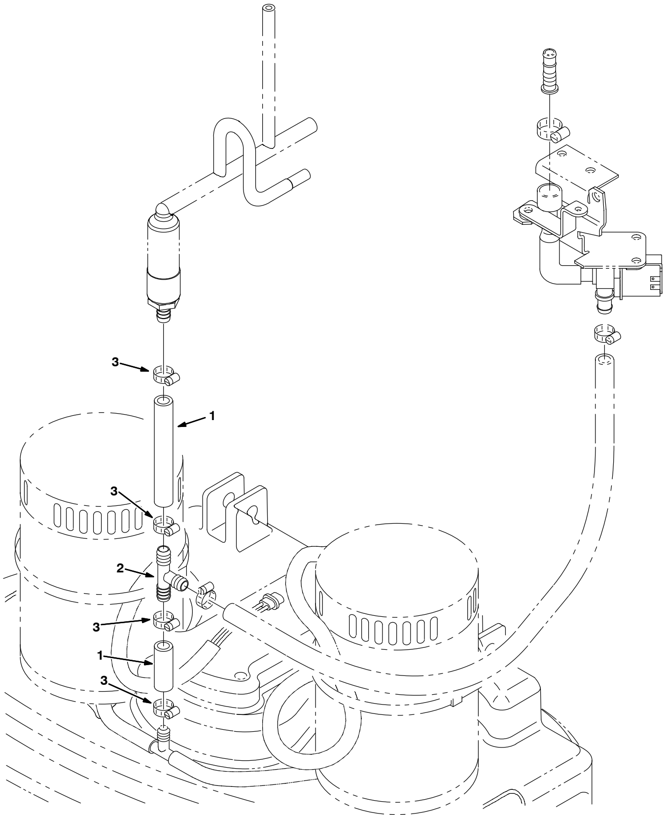
Fig. 4 – FaST Solution Supply Group, Disk Scrub Head (S/N 10000000 – 10361712)
