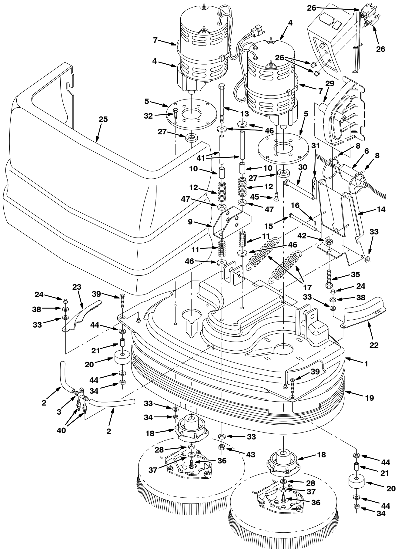
Fig. 13 – Scrub Head Kit, Model 900D, 900 mm (36 in) (S/N 10000000–10547659)
