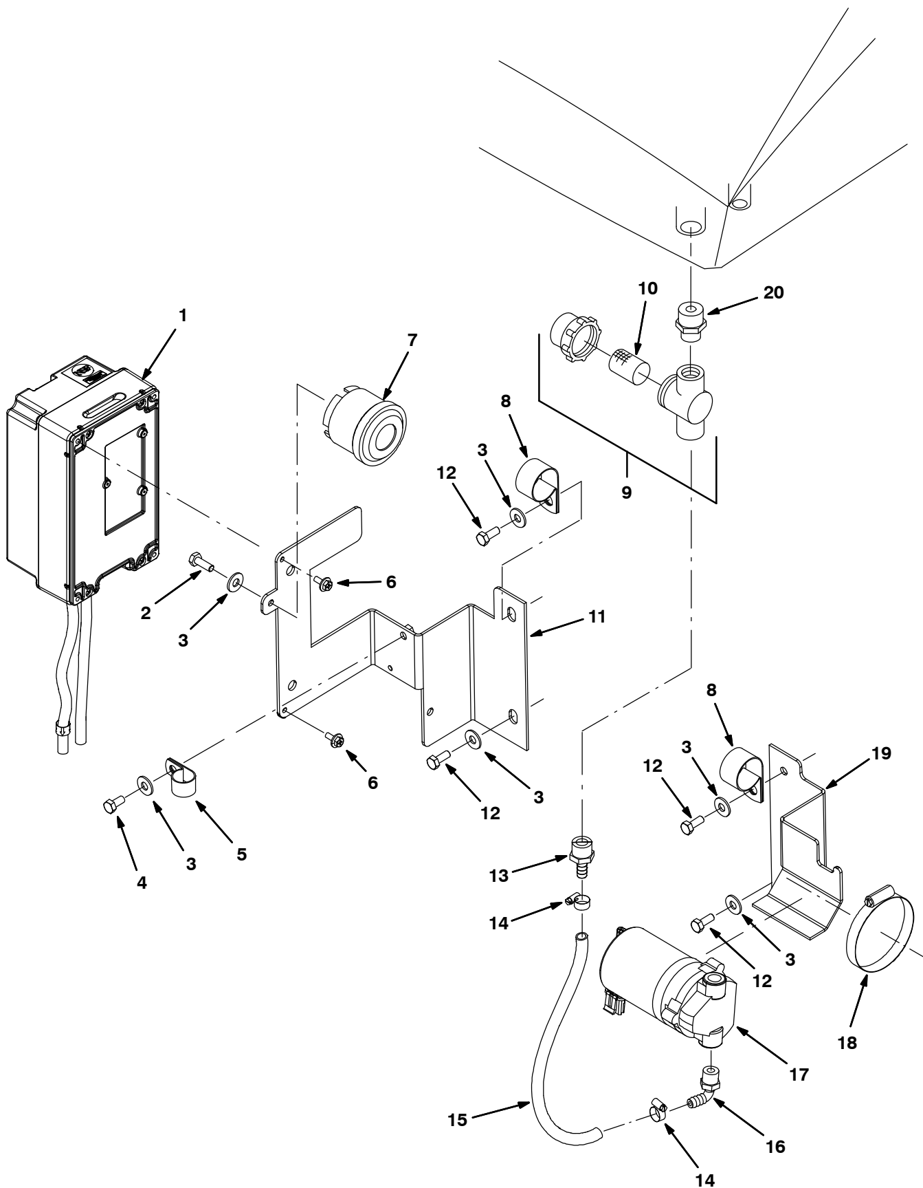
Fig. 13 – ec-H2O Solution Pump Group (S/N 10000000–10581869)
