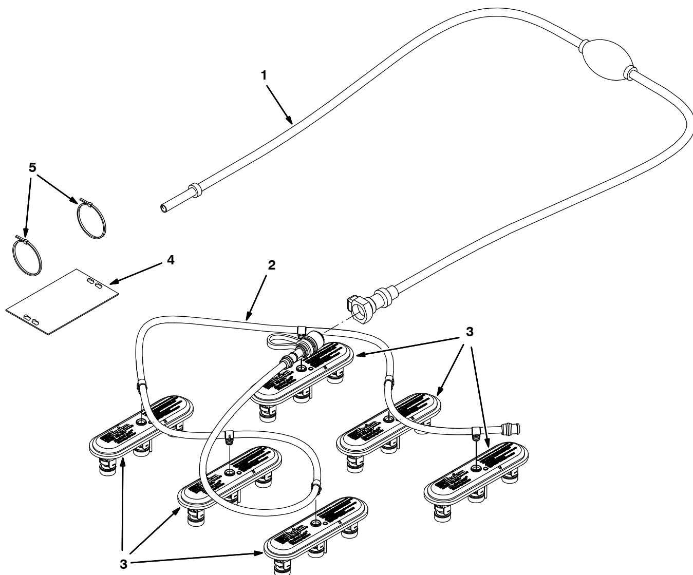
Fig. 42 – Hydrolink® Battery Watering System Kit
