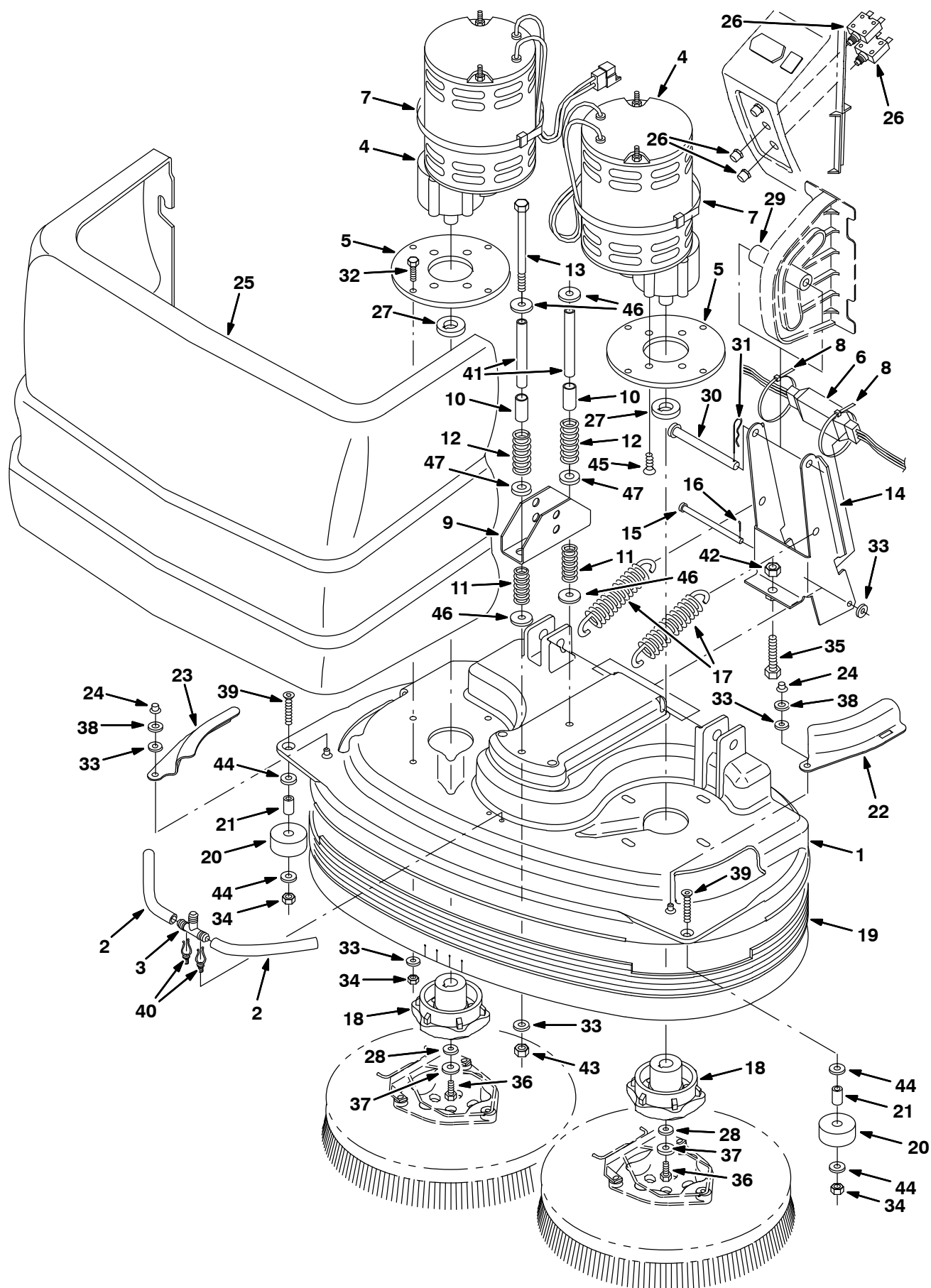
Fig. 15 – Scrub Head Kit, Model 800D Heavy Duty, 800 mm (32 in) (S/N 10000000–10547657)
