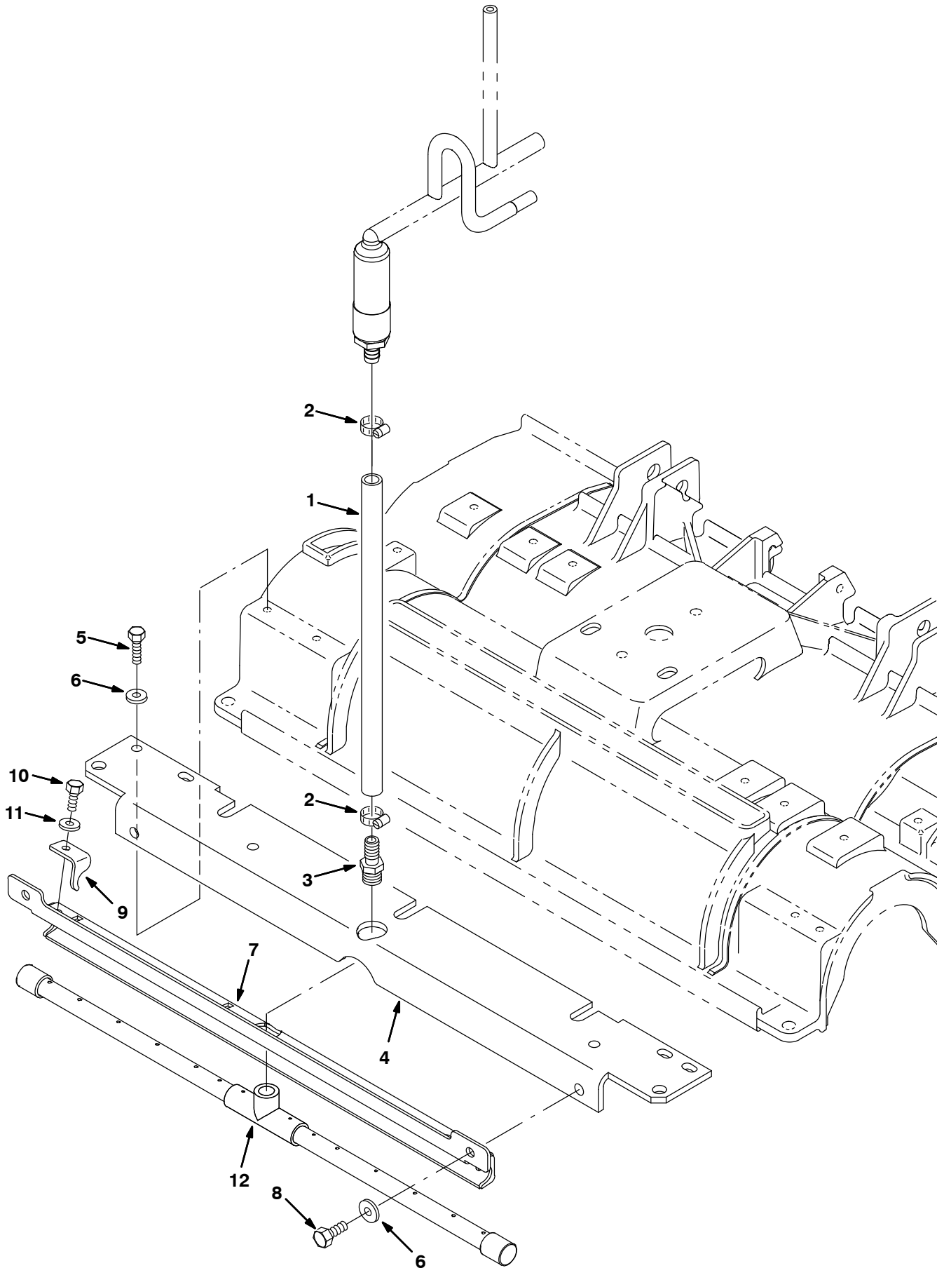
Fig. 6 – FaST Solution Supply Group, Model 700C / 800C Scrub Head (S/N 10000000 – 10361712)
