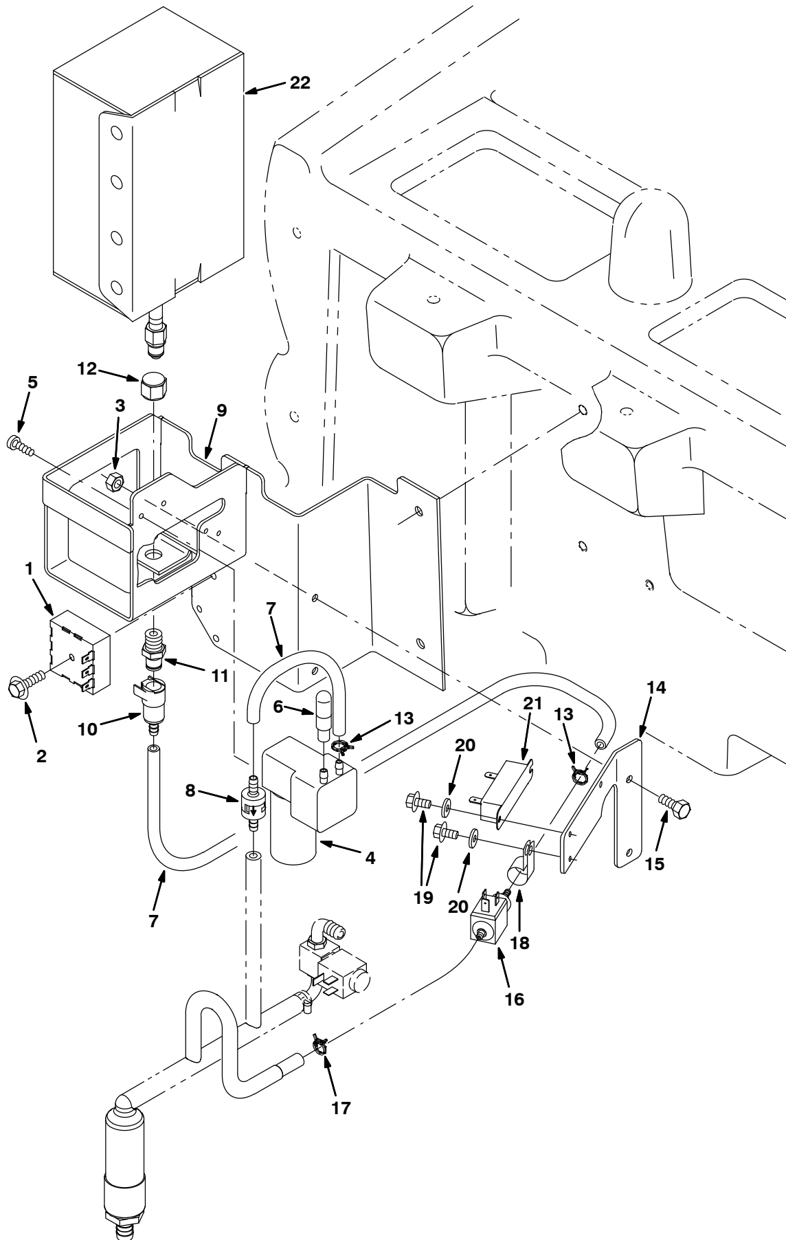
Fig. 2 – FaST Air Pump and Detergent Group (S/N 10000000 – 10361712)
