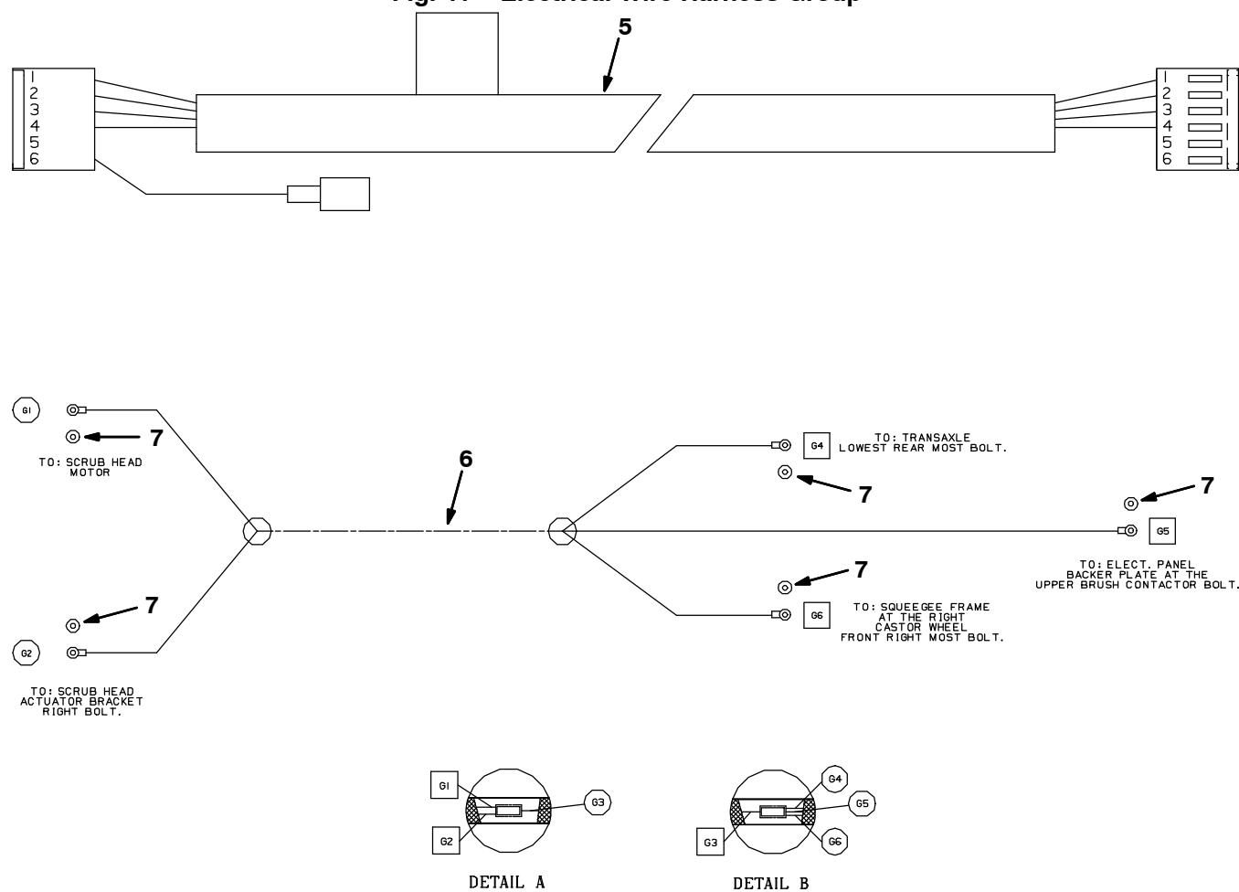
Fig. 41 – Electrical Wire Harness Group
