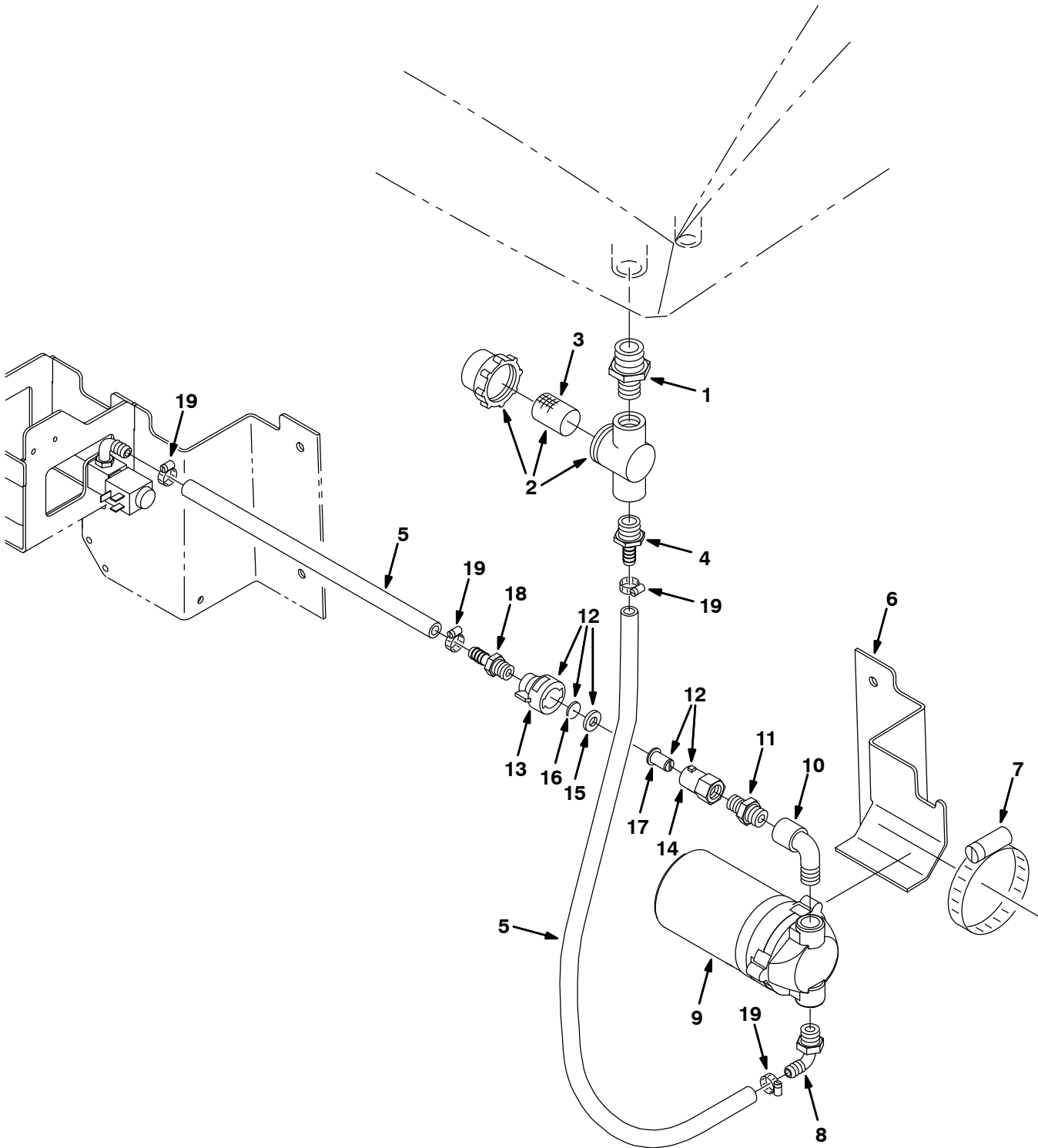
Fig. 9 – FaST Solution Pump Group (S/N 10000000 – 10361712)
