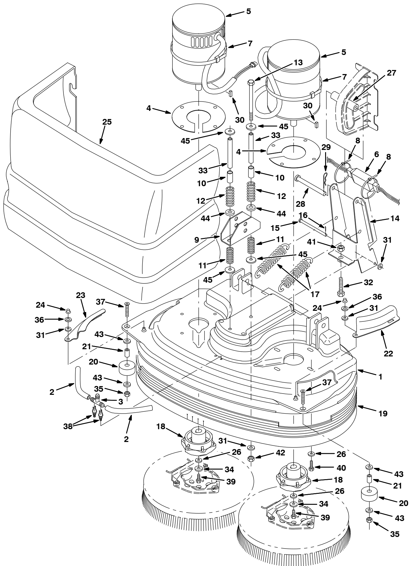
Fig. 11 – Scrub Head Kit, Model 800D, 800 mm (32 in) (S/N 10000000–10570246)
