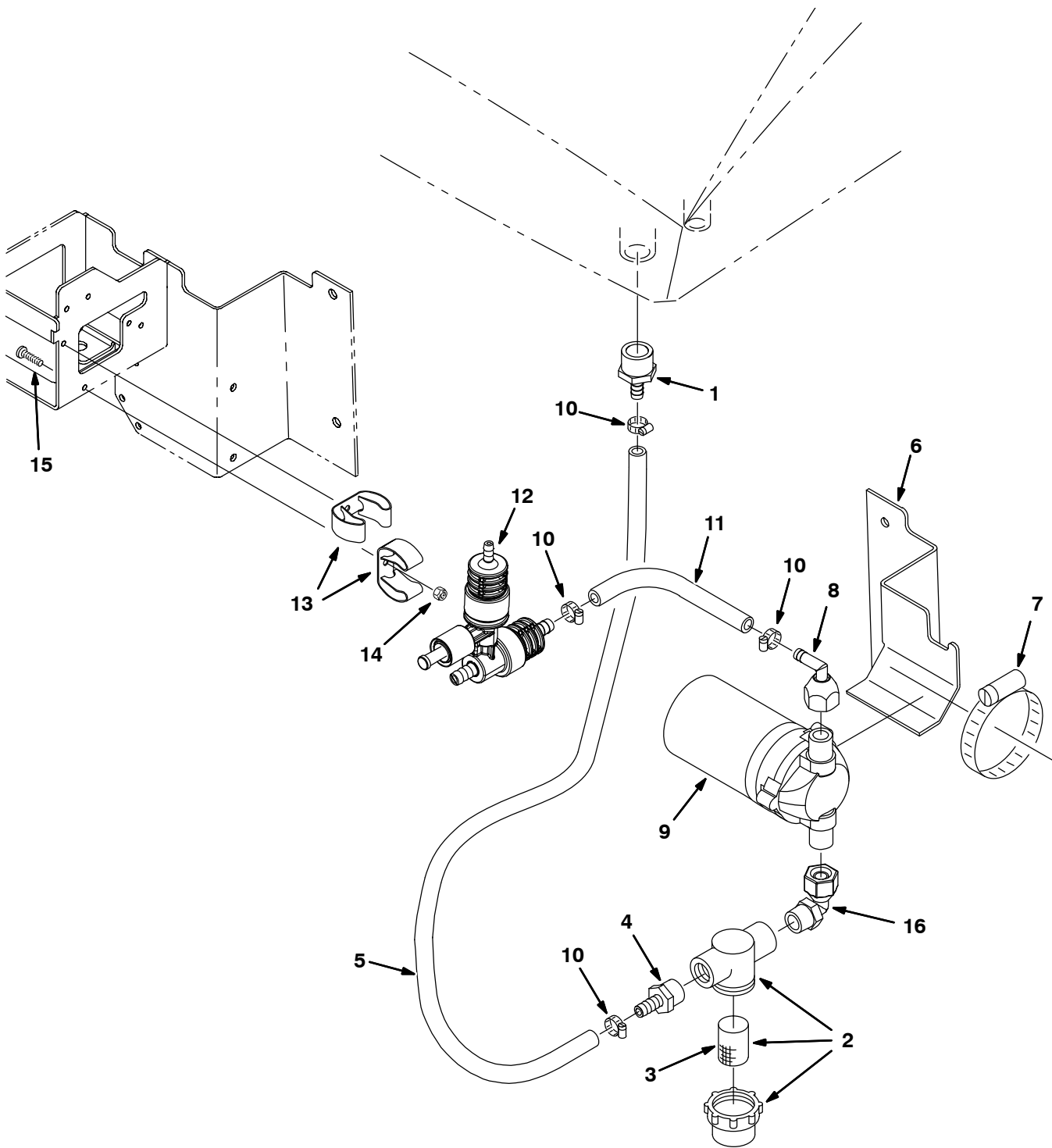
Fig. 11 – FaST Solution Pump Group (S/N 10581881– )
