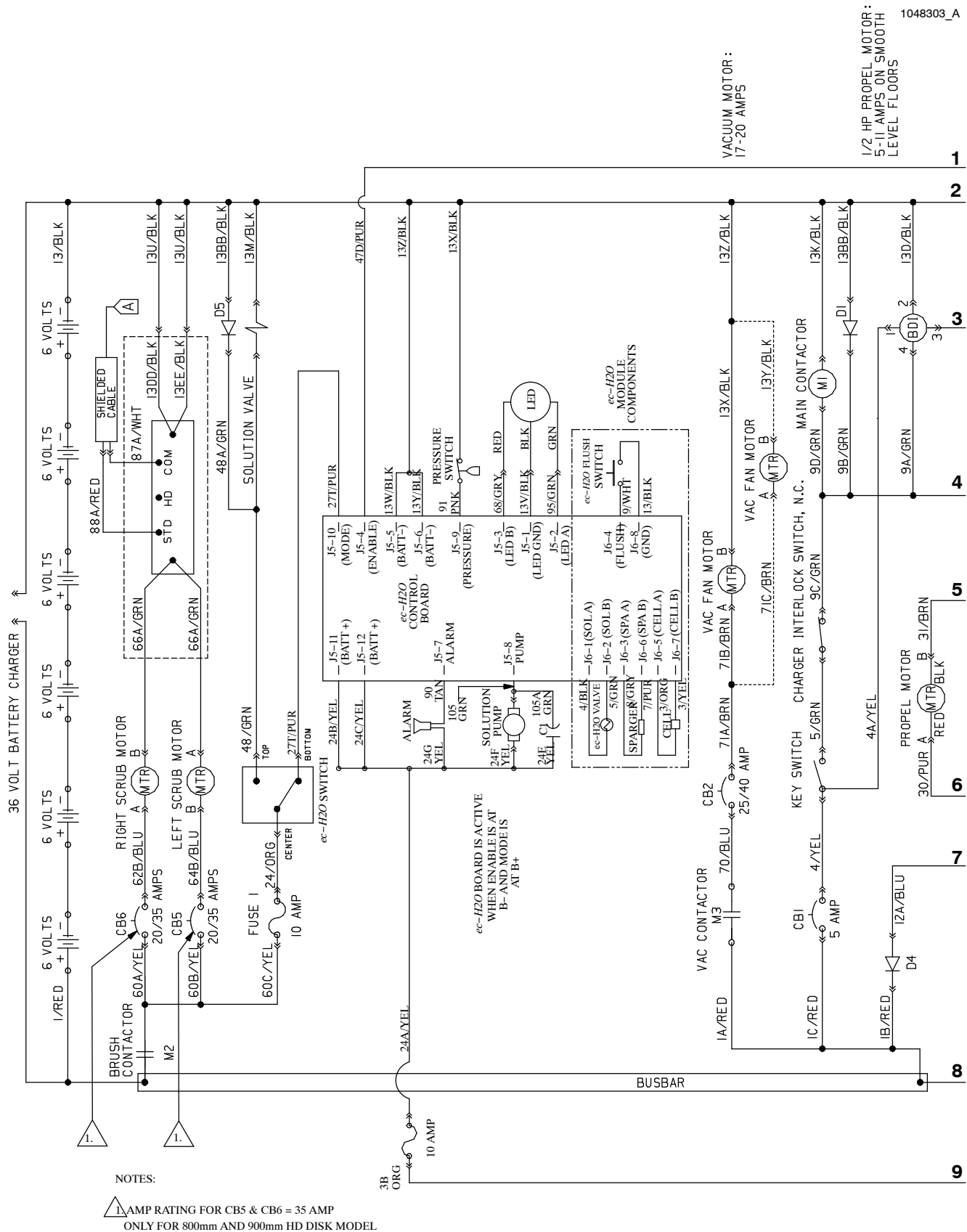
Fig. 39 – Electrical Schematic, ec-H2O Model (S/N 10403557–10741220)
