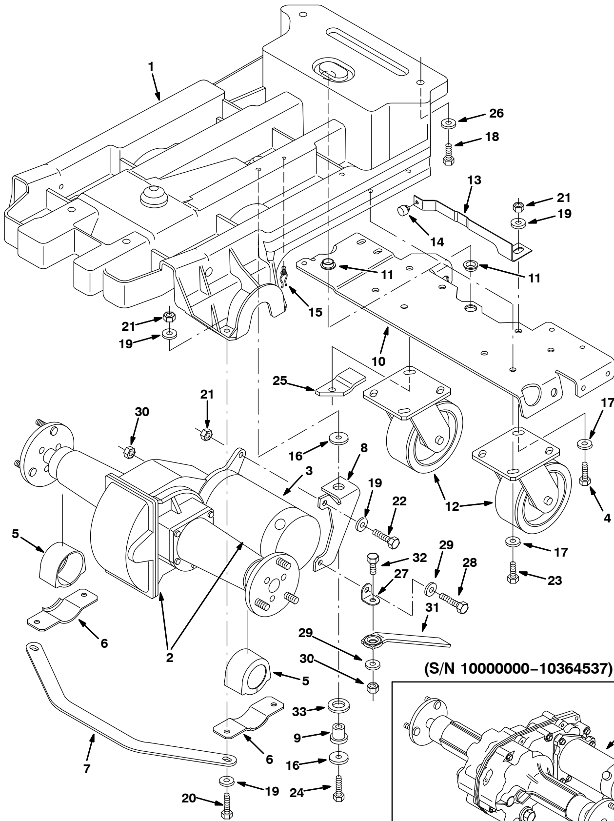
Fig. 5 – Main Frame and Drive Group (S/N 10000000–10705714)
