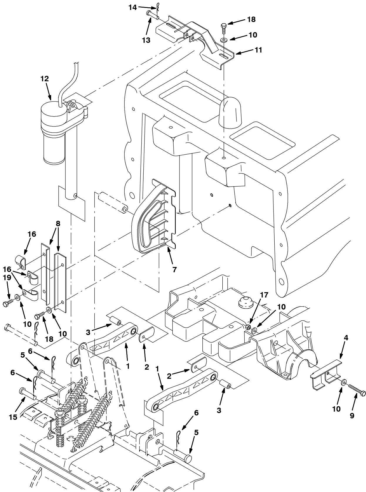
Fig. 7 - Scrub Head Lift Group
