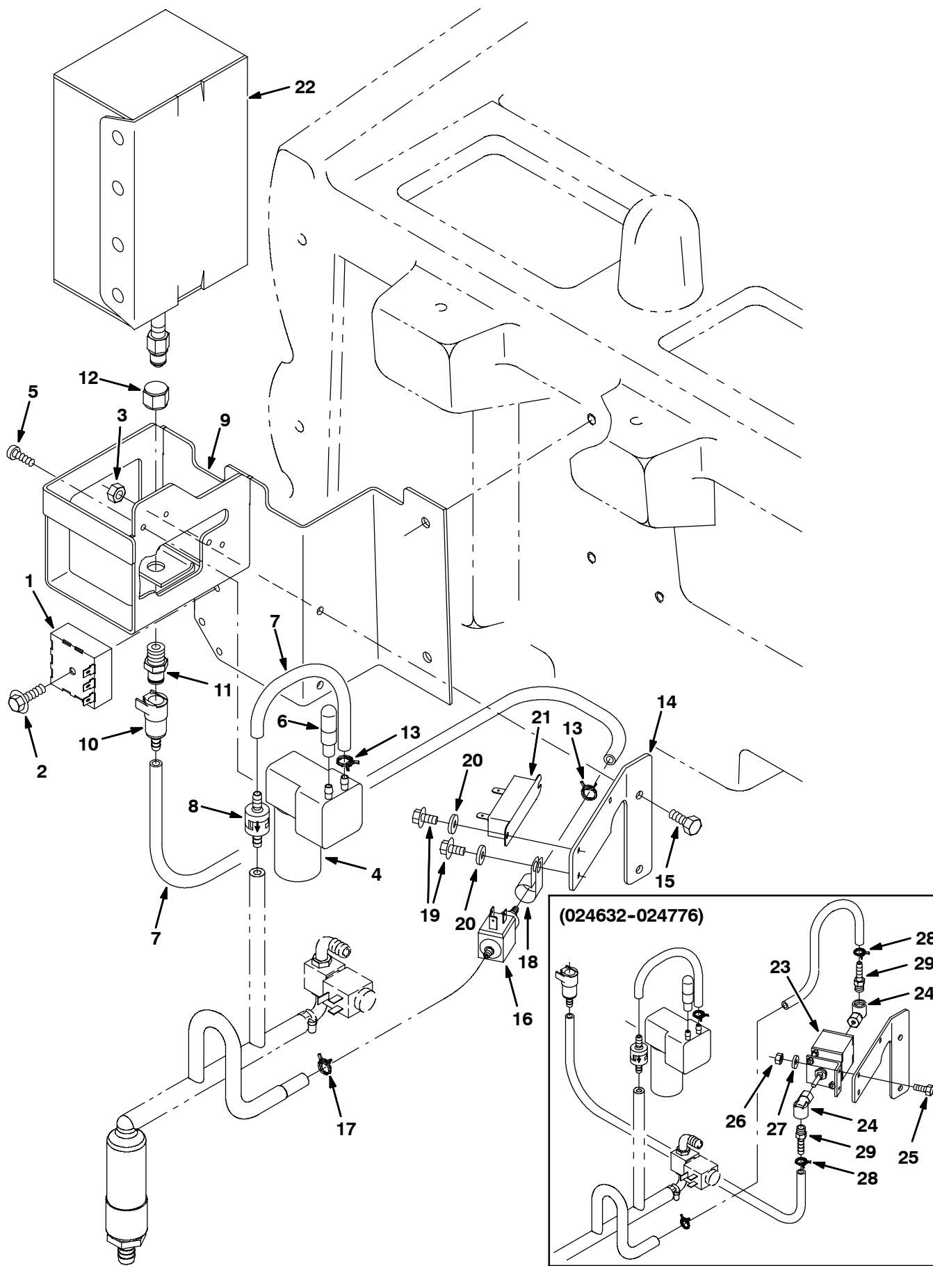
Fig. 23 - FaST Air Pump and Detergent Group (024028- )
