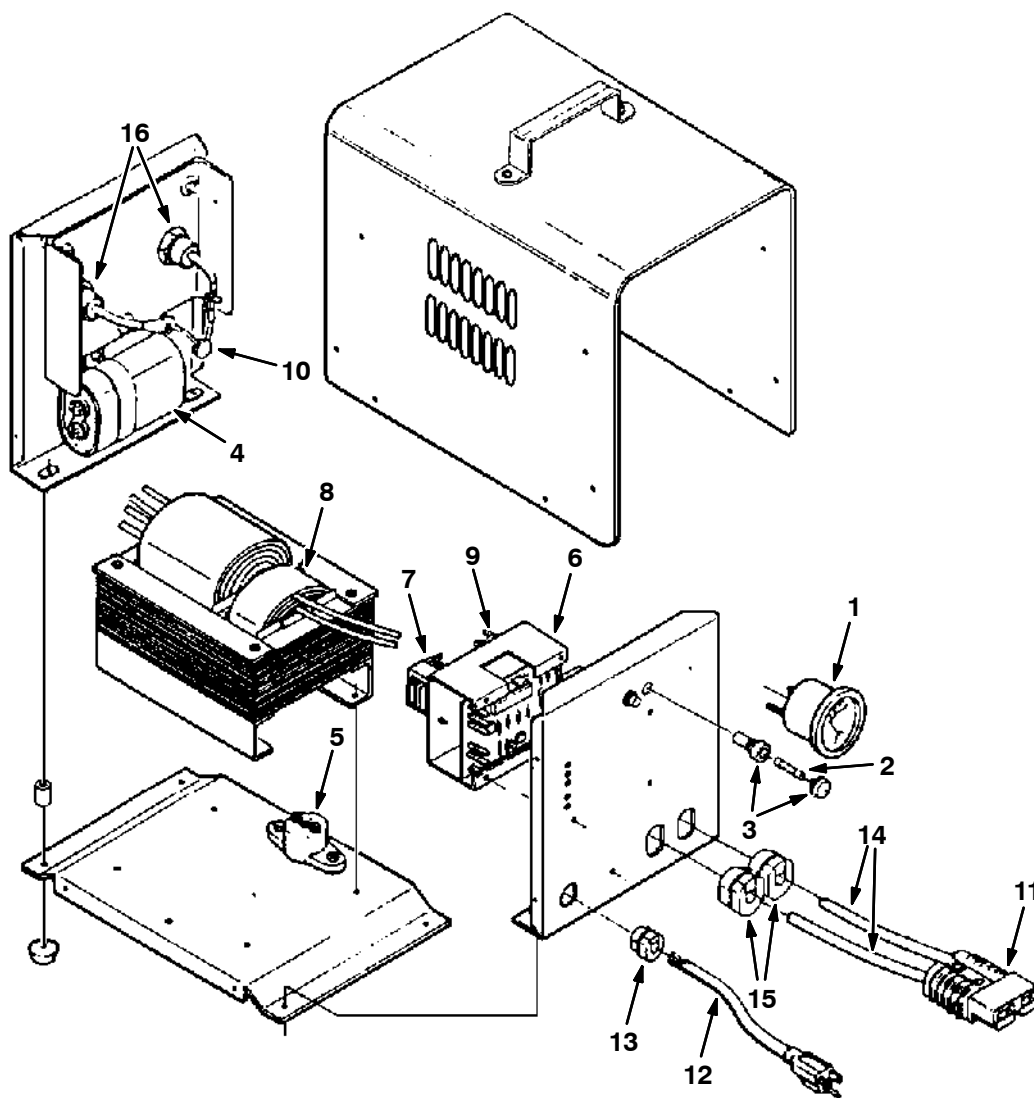
Fig. 16 - Battery Charger Breakdown, 60 Hz, 115V (305 Ah batteries), 222594
