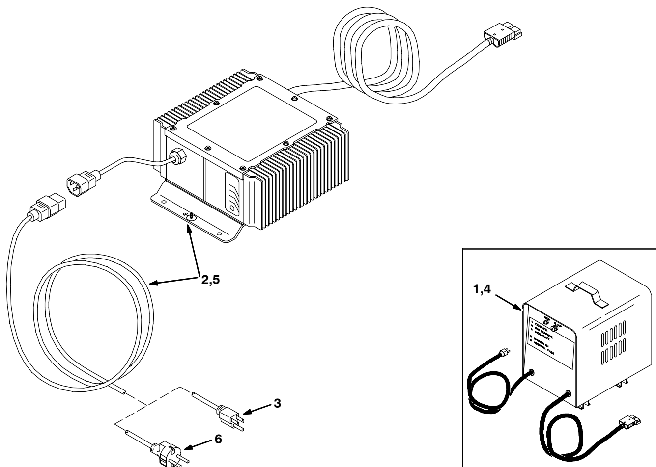
Fig. 17 - Battery Charger Group
