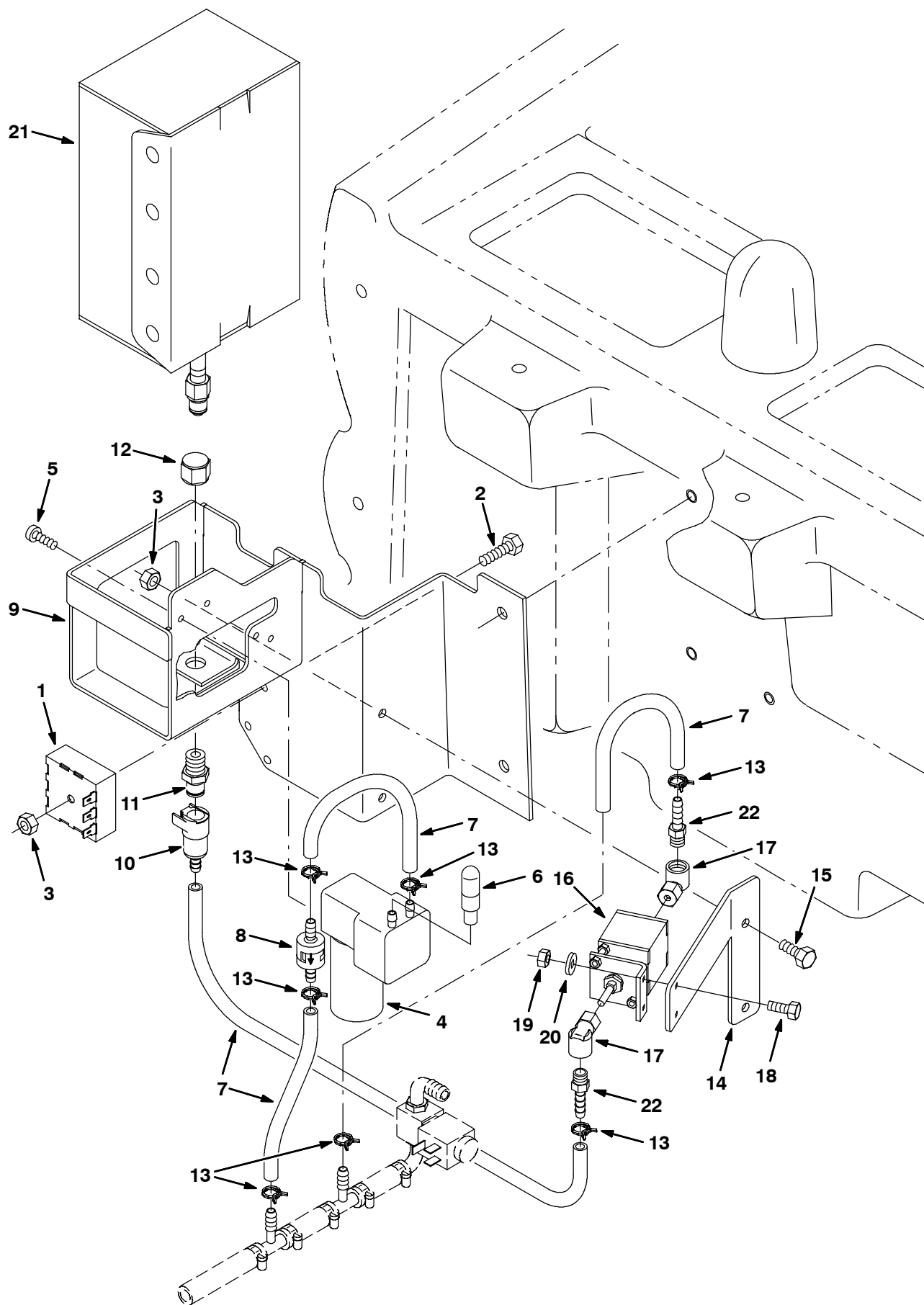
Fig. 22 - FaST Air Pump and Detergent Group (022741-024027)
