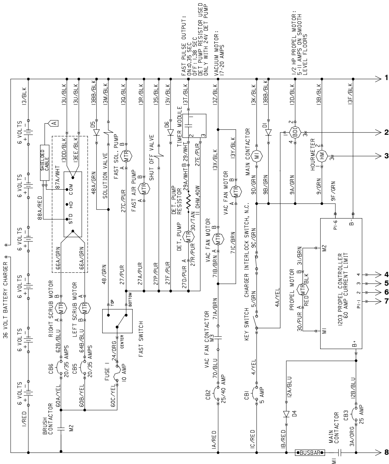
Fig. 37 - Electrical Schematic (022000- )
