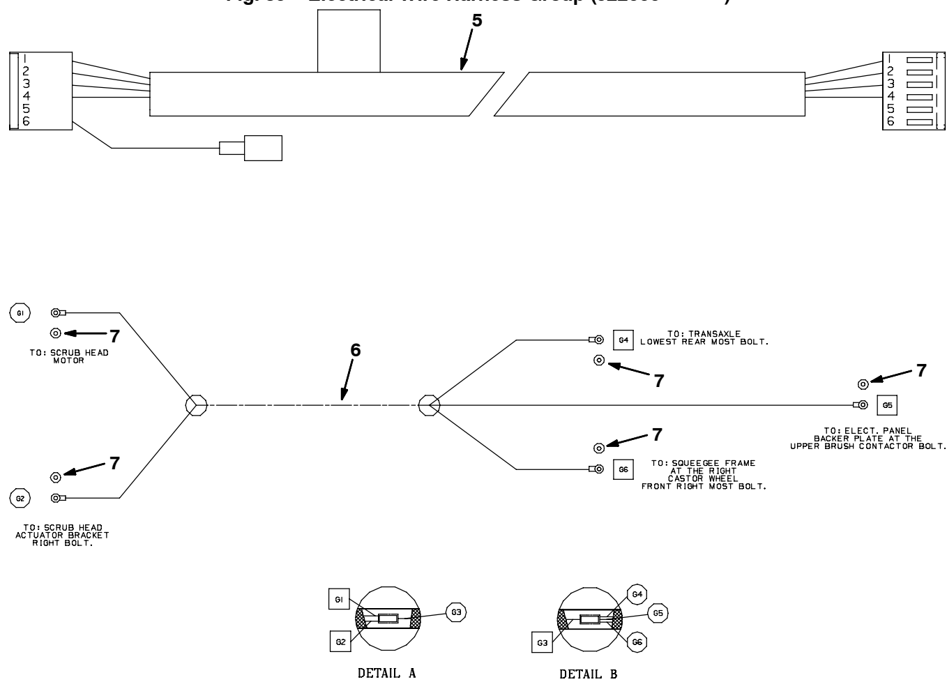
Fig. 39 - Electrical Wire Harness Group (022000- )
