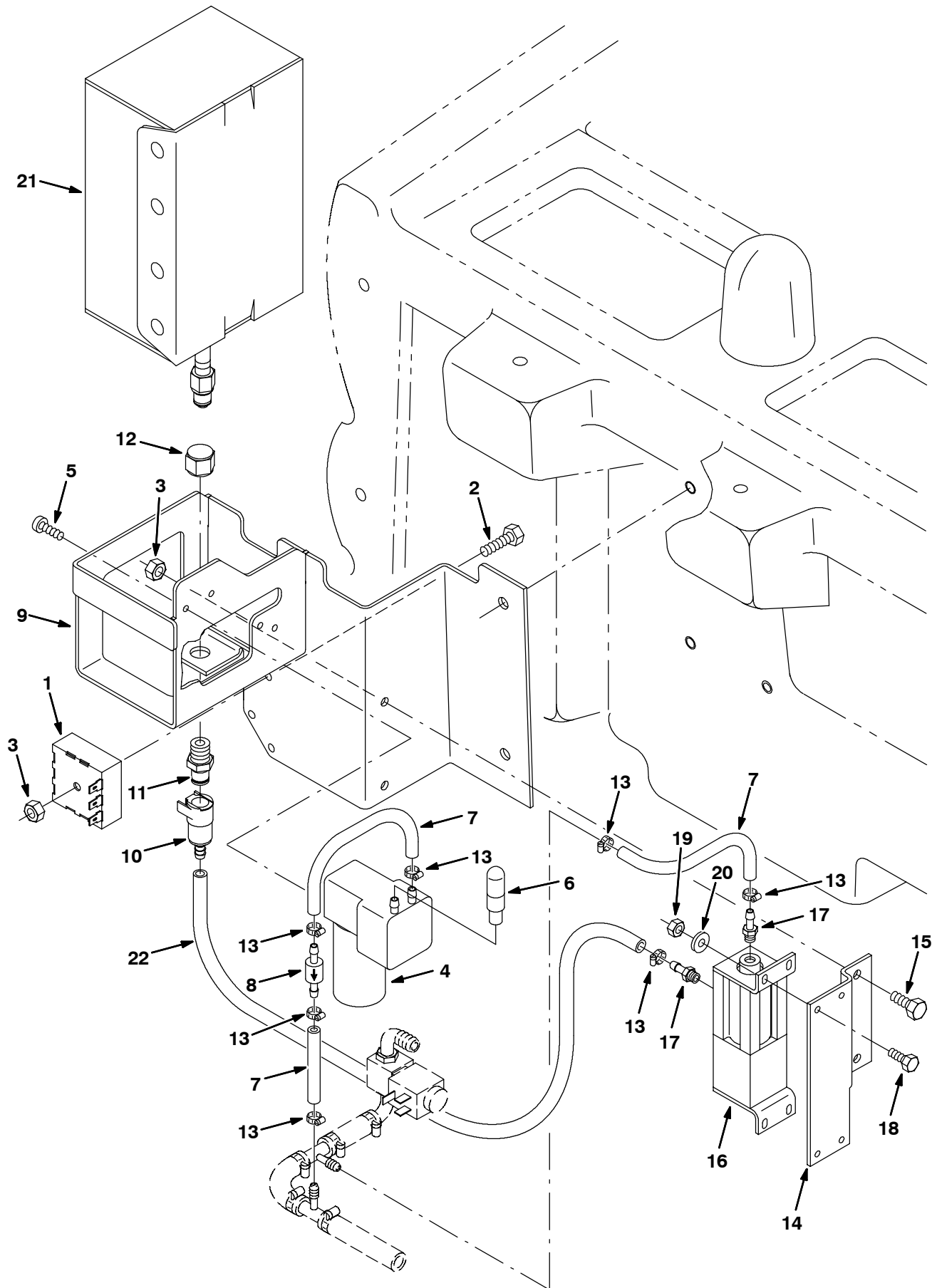
Fig. 21 - FaST Air Pump and Detergent Group (000000-022740)
