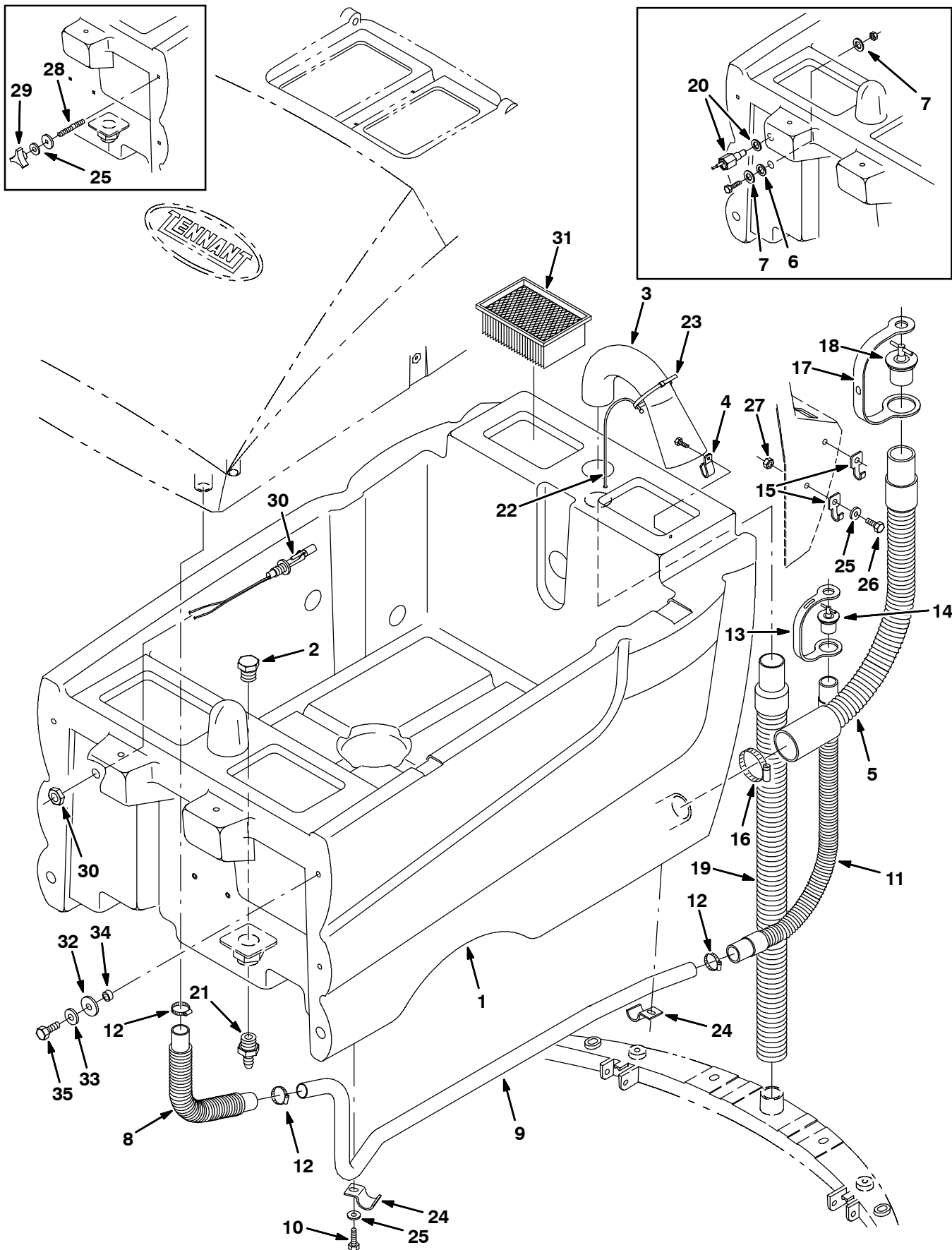
Fig. 18 - Recovery Tank Group (000000-022108)
