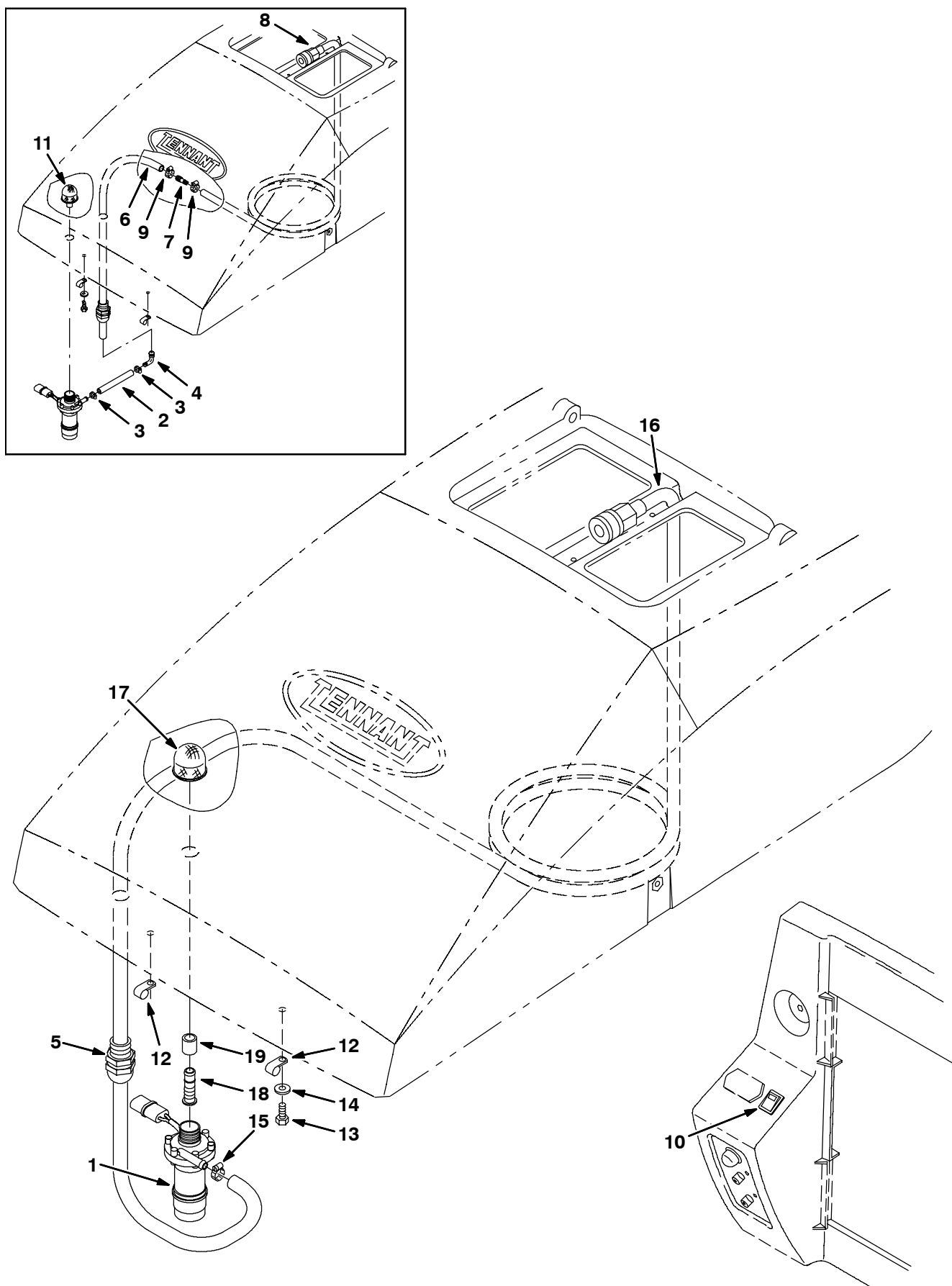
Fig. 5 - Power Wand Pump and Fittings Group
