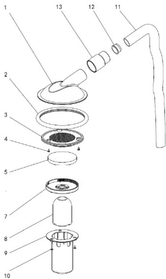
6. Float Assembly
