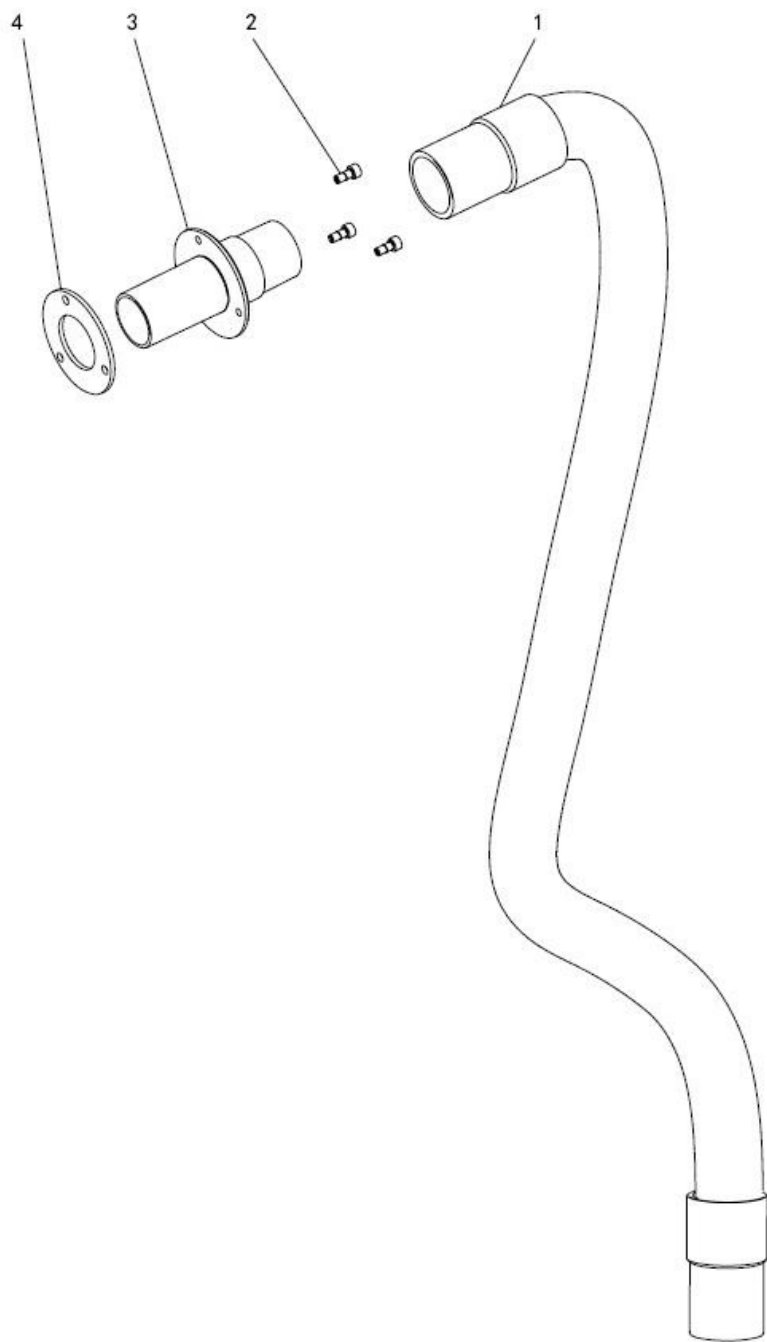
13. Vacuum Hose Assembly
