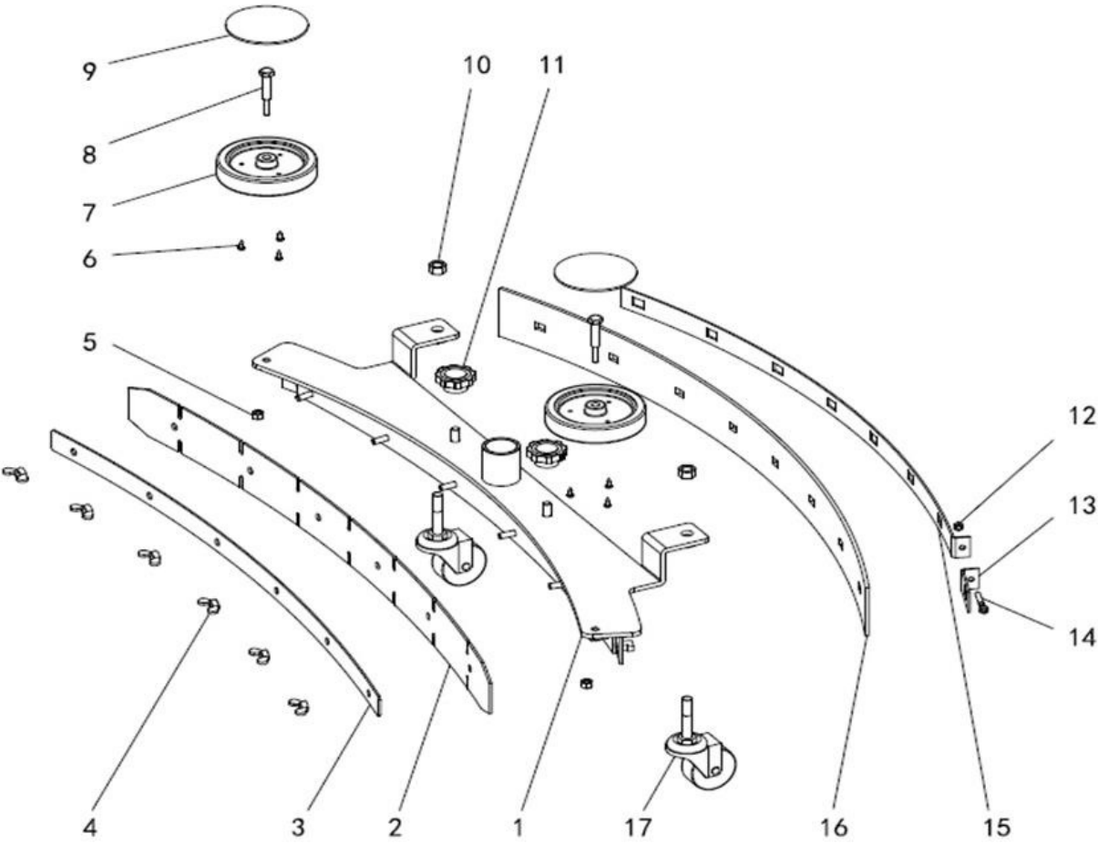
9. Squeegee Assembly Rendered by LeadVenture, Inc.
