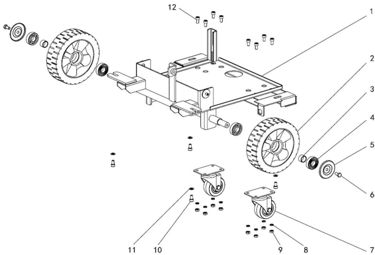
1. Chassis Assembly
