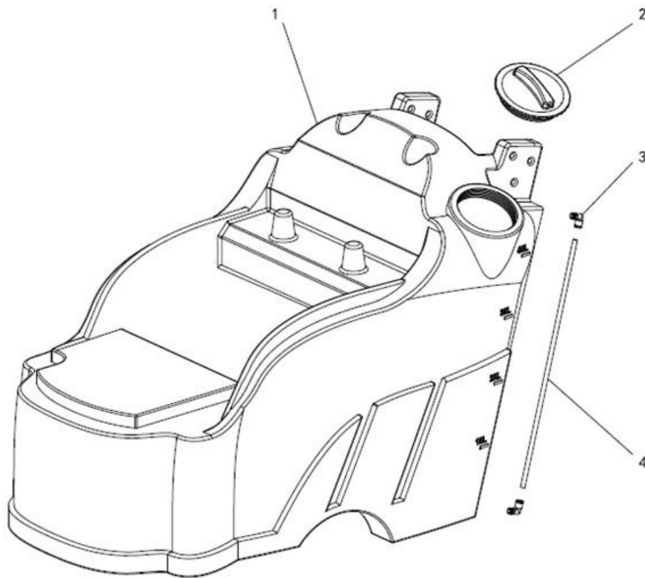
4. Solution Tank
