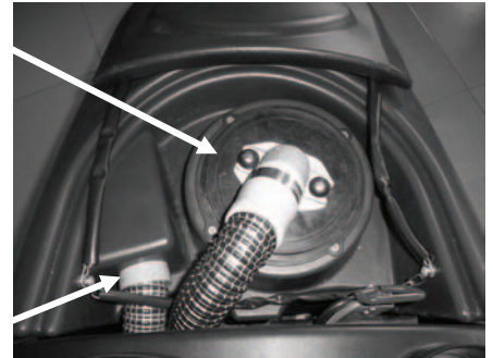
Vacuum Cover
