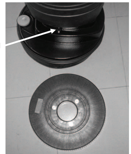
Splash Guard Height Adjusting Knob
