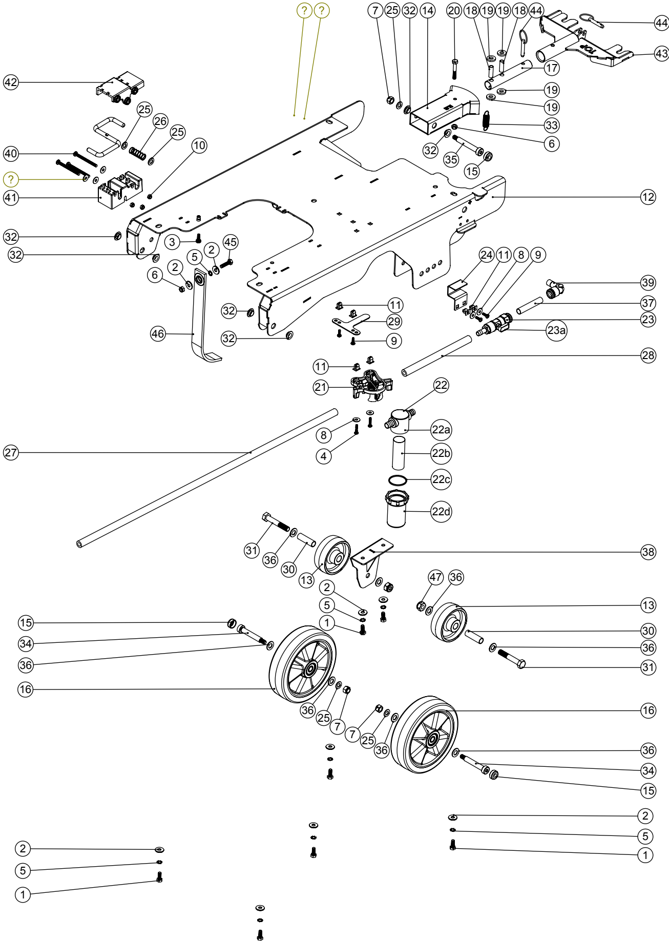
EGB1120 Chassis.pdf
