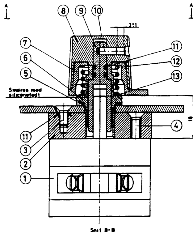
START/STOP SWITCH
