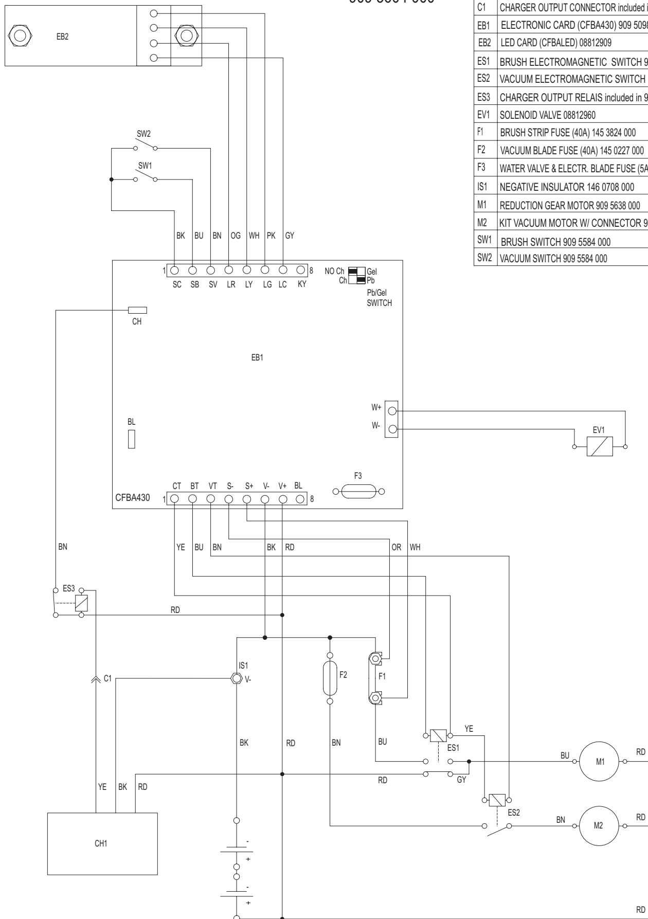
WIRING DIAGRAM 909 5604 000
